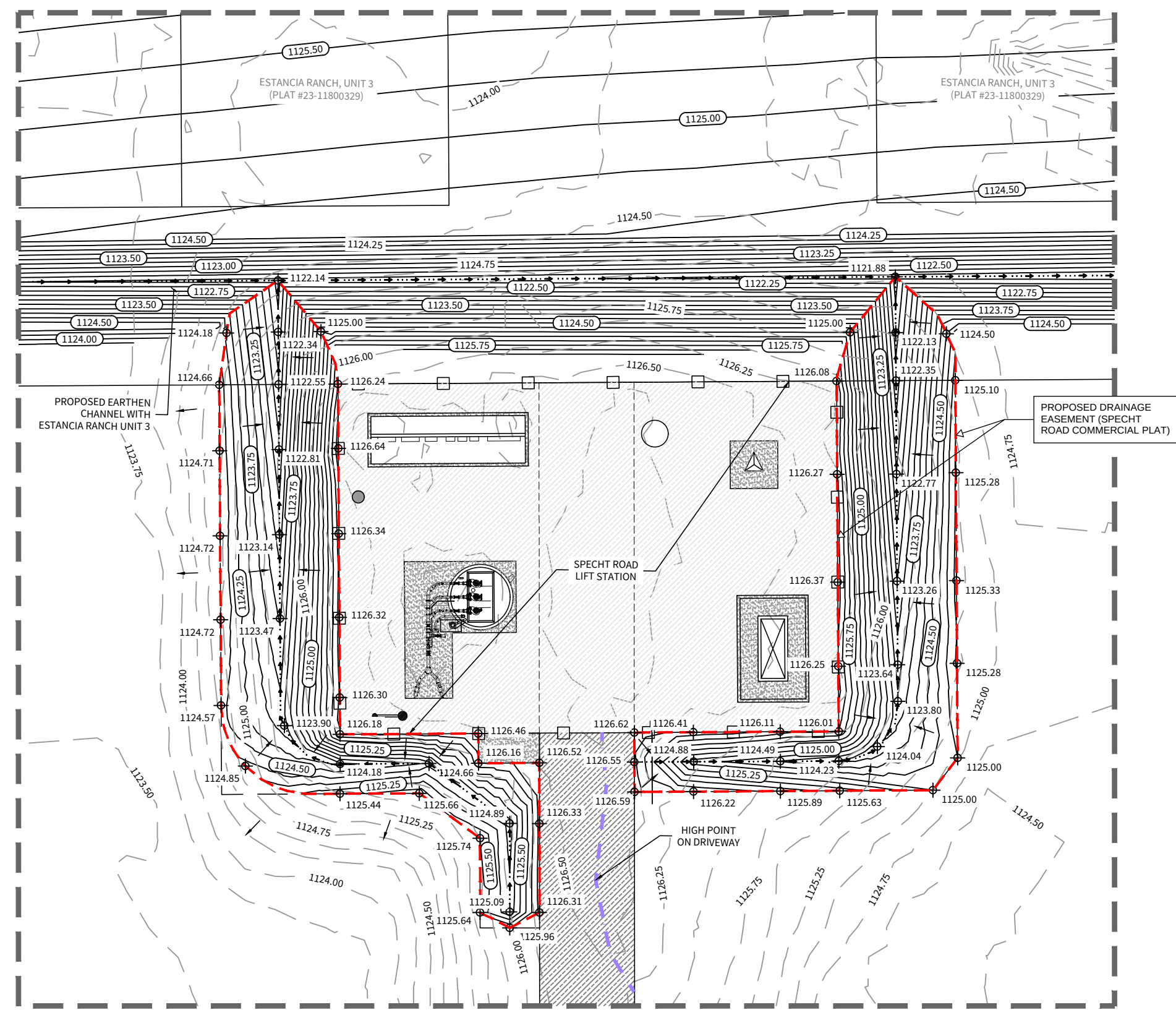
DETAIL "A" SCALE 1" = 20'
