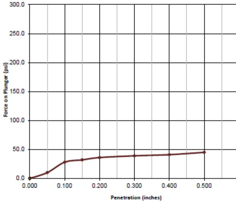
CBR Results
