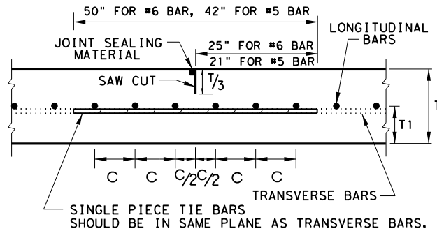
LONGITUDINAL CONTRACTION JOINT SECTION Z - Z
