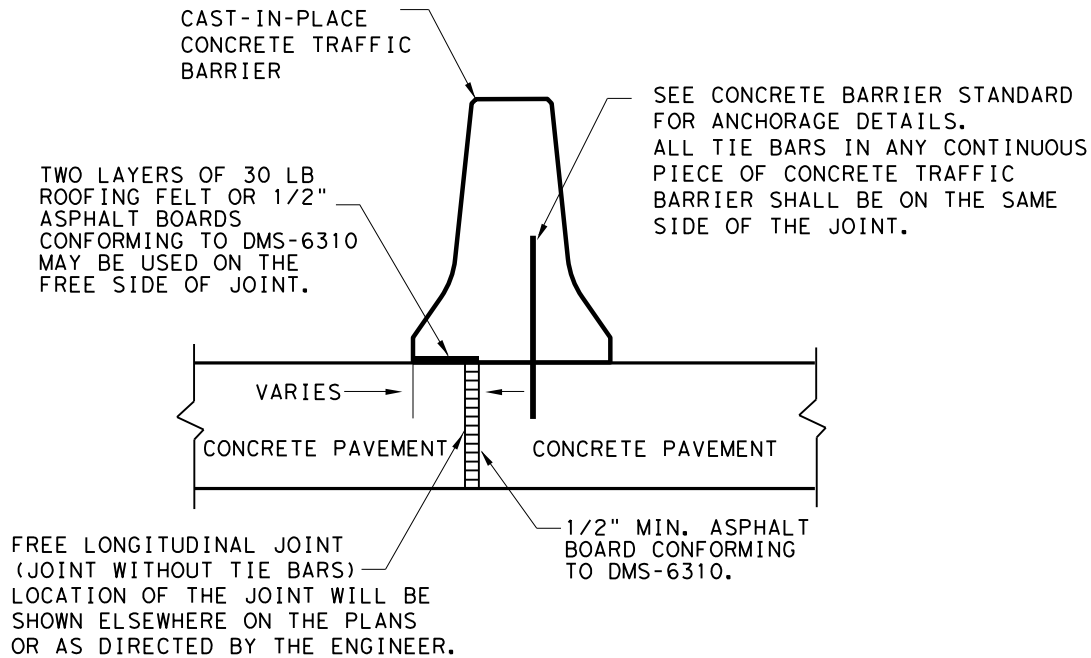
FREE LONGITUDINAL JOINT DETAIL
