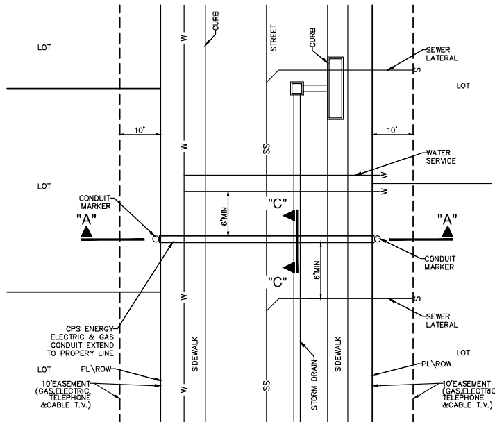
CONDUIT PLAN CROSSING NOT TO SCALE
