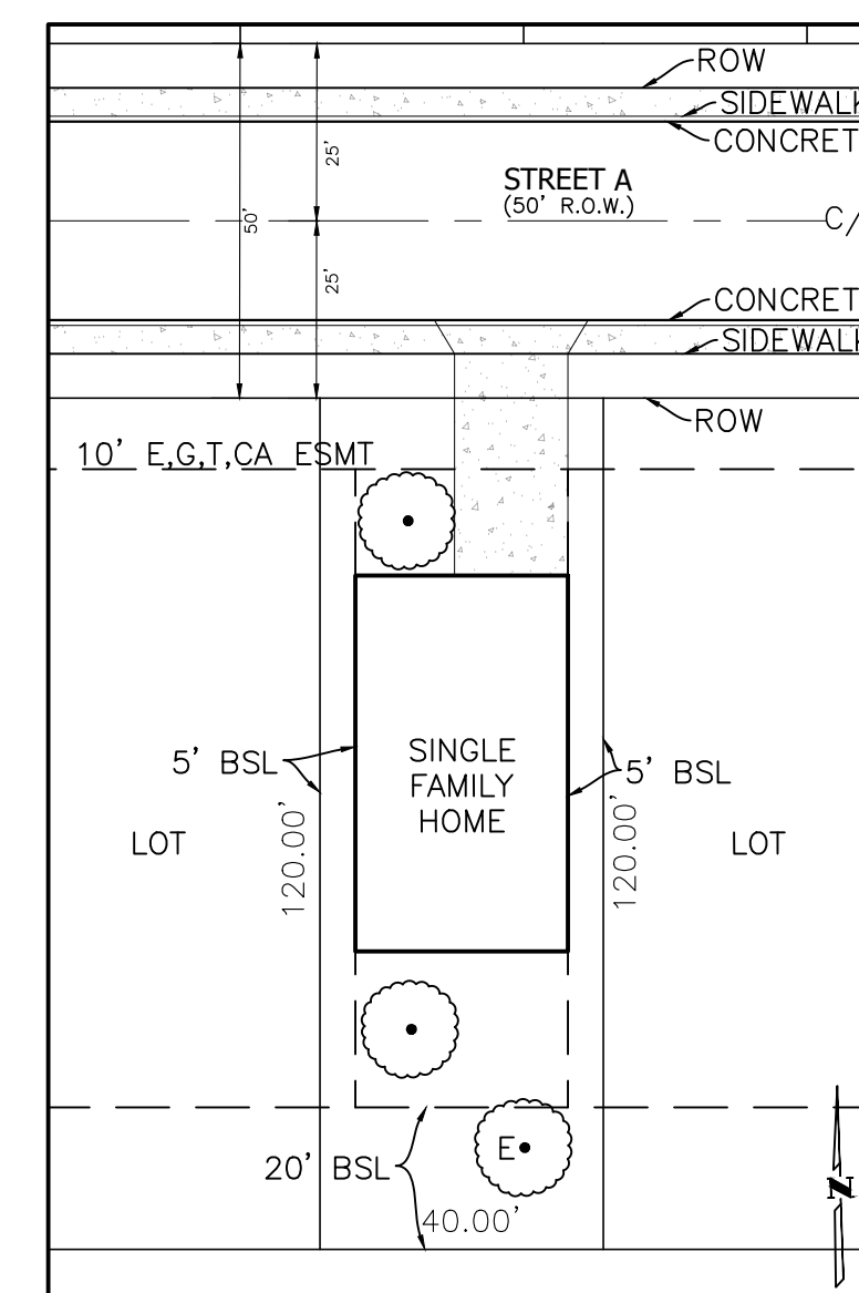
TYPICAL LOT LAYOUT SCALE 1:30
