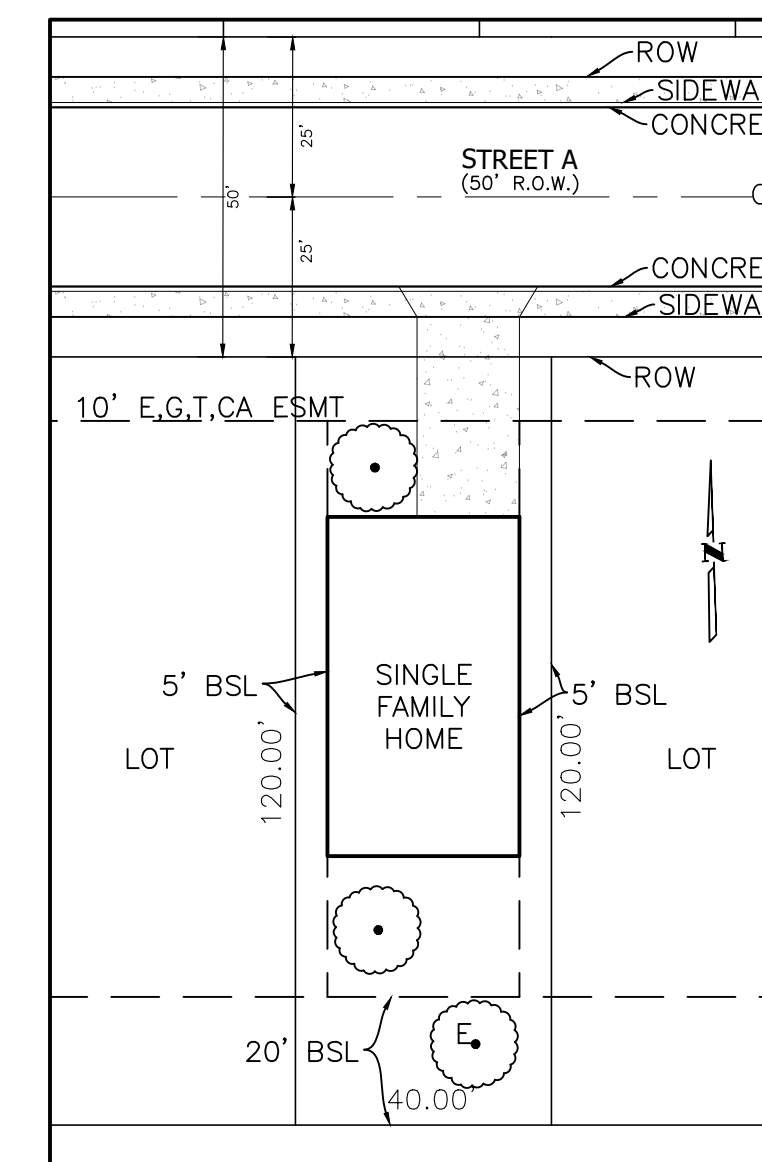
TYPICAL LOT LAYOUT SCALE 1:30
