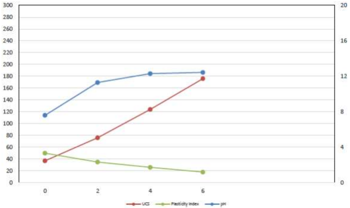
Lime Series Curves
