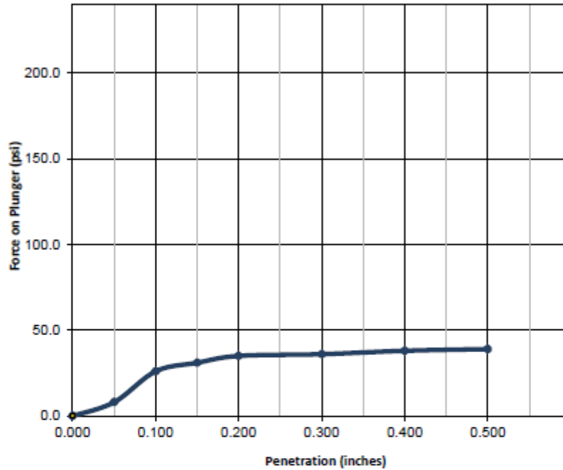
Load Penetration Curve
