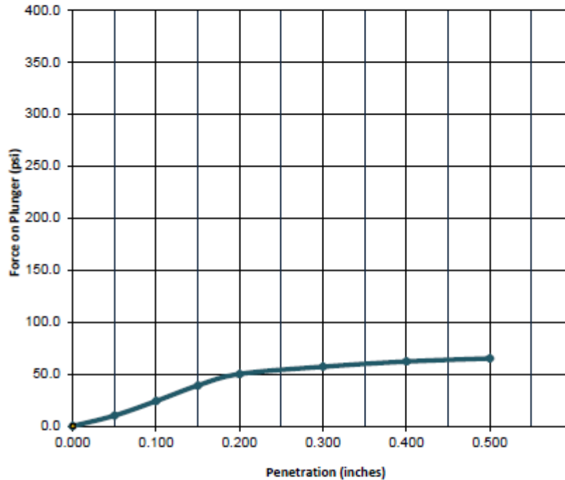
Load Penetration Curve
