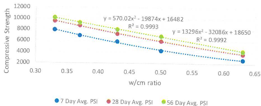
w/cm ratio vs Compressive Strength
